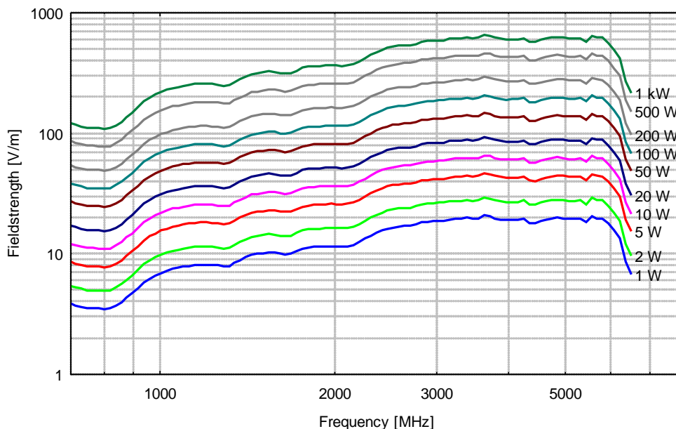
BBHA 9120 J Input Power, Dist. Aperture-EuT: 3 m
