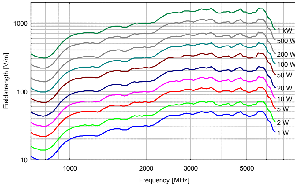
BBHA 9120 J Input Power, Dist. Aperture-EuT: 1 m
